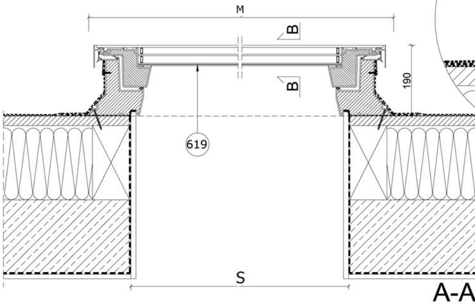
619-DEF DU6 Flat Roof Window, electrically opened, with transparent dome, glazing unit DU6
